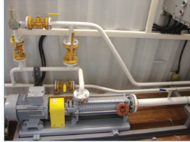
Side Channel Multistage LPG pump Installed In 20 Foot Container Filling Hall
