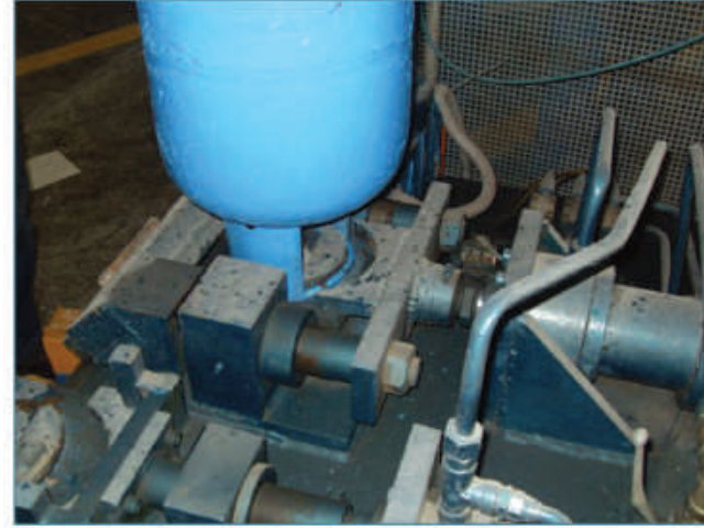
Hydraulic Operated Cylinders Handles Straightening Machine
